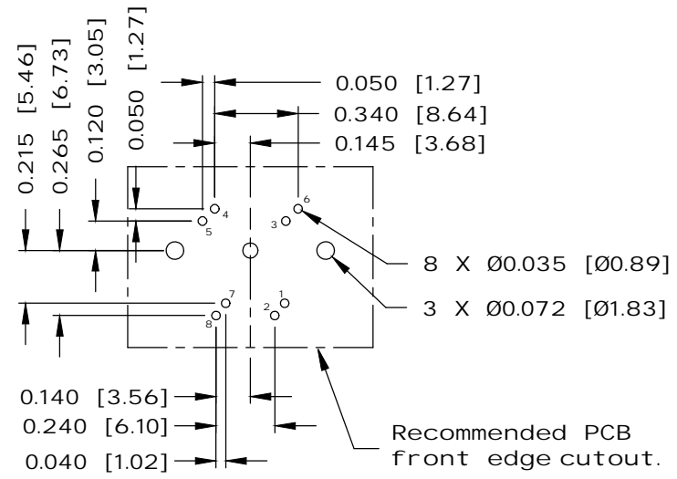
PCB RECOMMENDED HOLE LAYOUT (COMPONENT SIDE VIEW)
